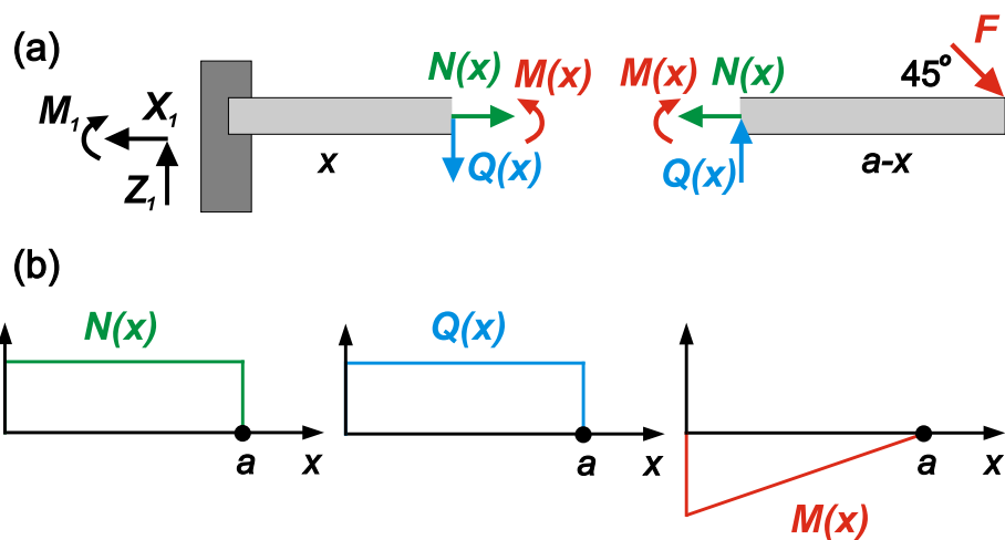
Figure 3.1: (a) Free body diagram for a beam with intermediate cut. (b) Internal forces and moments diagrams as functions of coordinate x .
