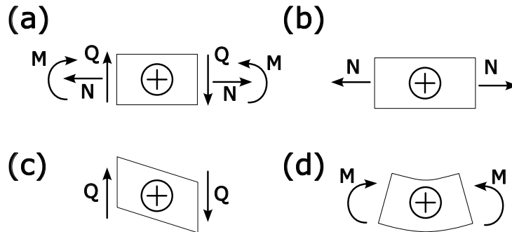
Figure 2.5: (a) Sign conventions for normal force N , shear force Q and bending moment M . Deformations caused by (b) normal force, (c) shear force and (d) bending moment.
