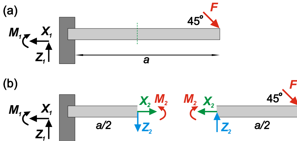
Figure 2.6: Reaction forces and moments in the beam fixed on the left side and subjected to inclined point load on the right.
